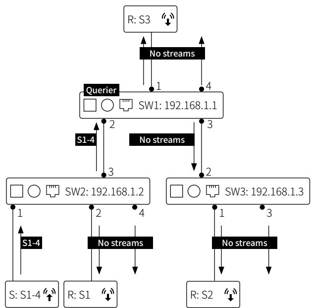
Figure 12: Incorrect IGMP implementation, Unknown Flooding disabled
