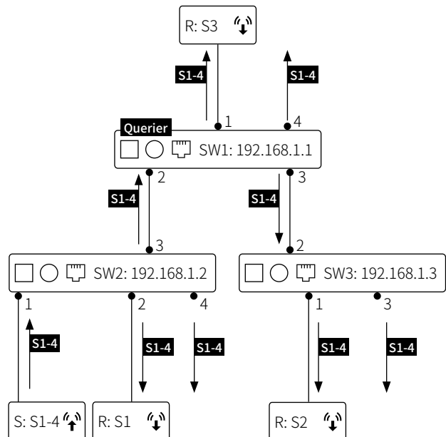
Figure 10: Incorrect IGMP implementation
